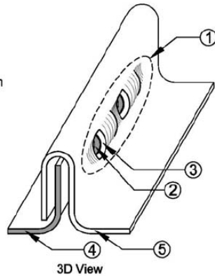
4e. Verco VSC 2 Connection
