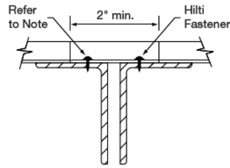
4b. Steel Deck Endlap Condition
