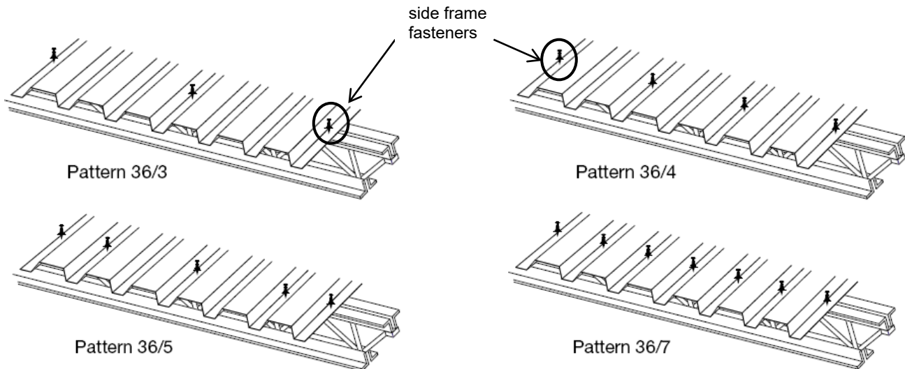
FIGURE 3a—COMMON FRAME FASTENER PATTERNS
