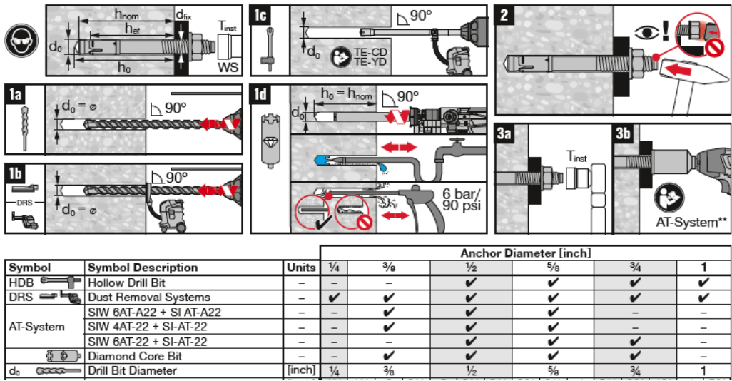
FIGURE 7—INSTALLATION INSTRUCTIONS
