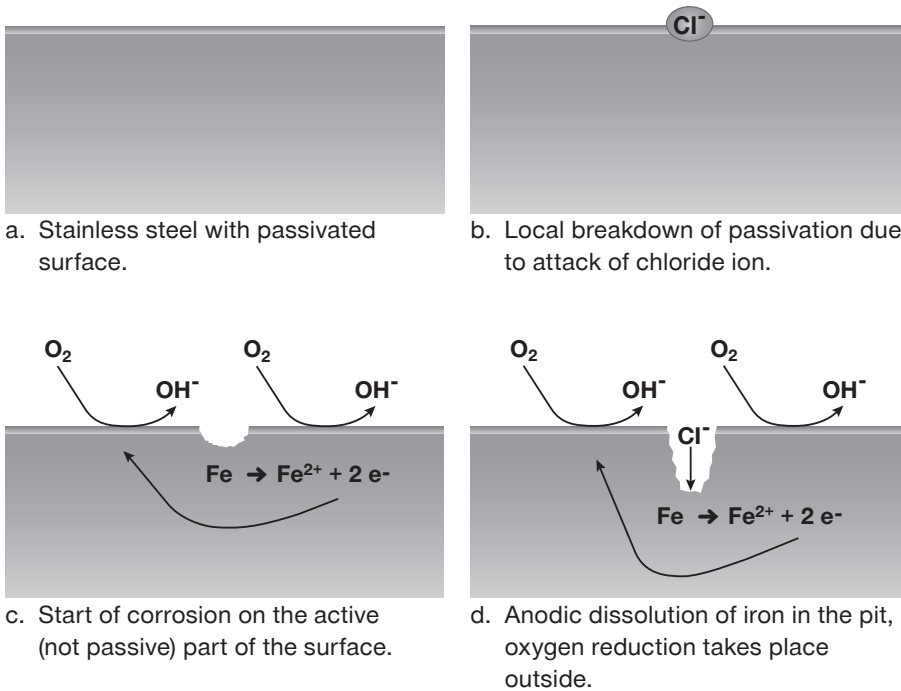
Fig. 6: Phases of pitting corrosion on stainless steel.
