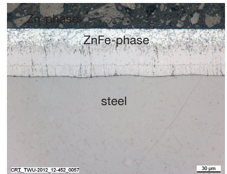
Fig. 30: Micrograph of hot-dip galvanized steel.
