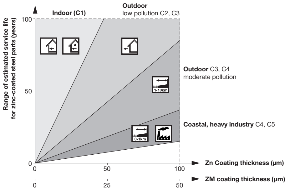
Fig. 29: Typical service life of Zn- and ZM-coated steel across various environments, with typical corresponding C-classes categories indicated.
