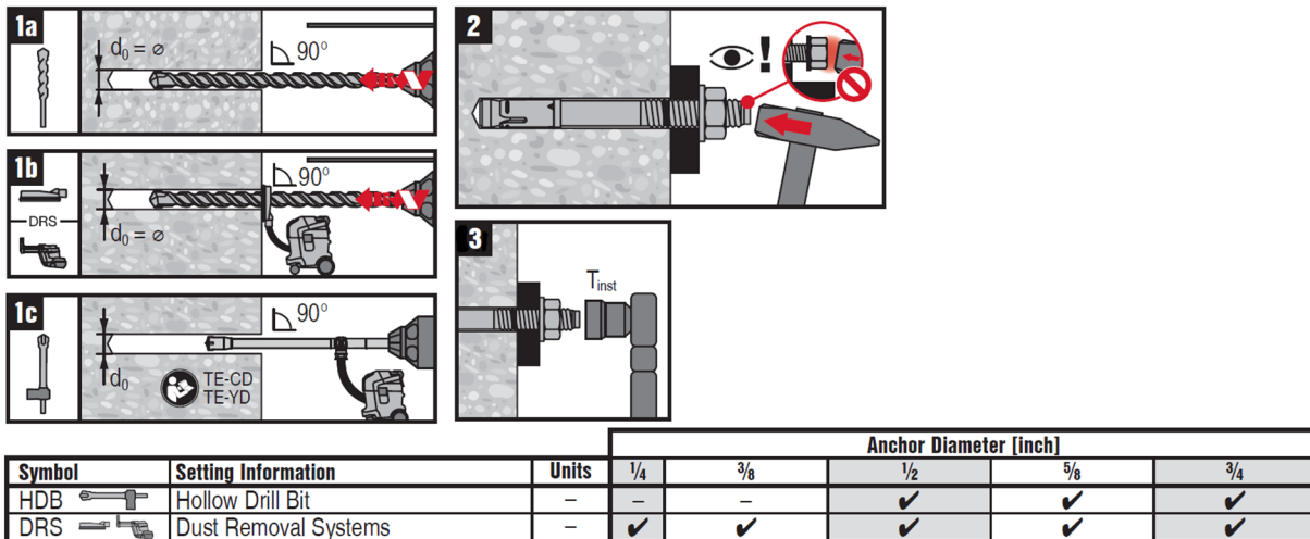
FIGURE 7—INSTALLATION INSTRUCTIONS
