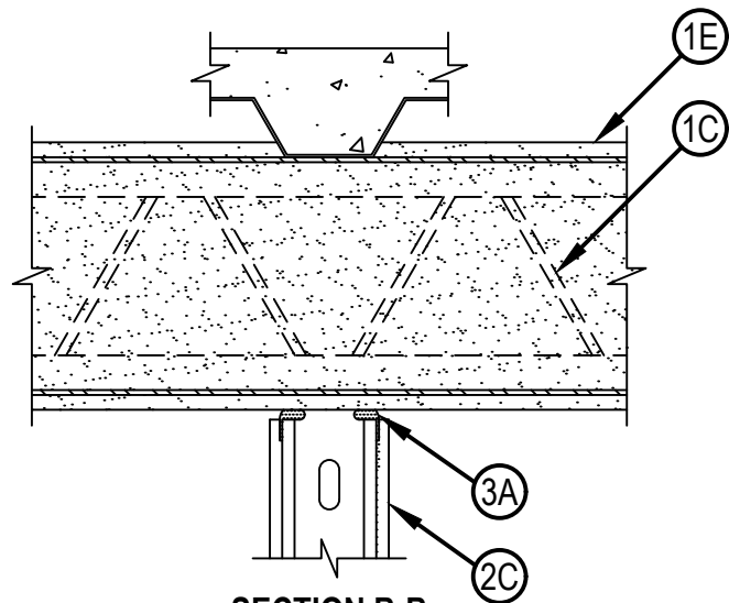
SECTION B-B
